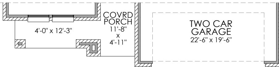
OPTIONAL "ELEVATION - B" FRONT PORCH ( ADDS 102 TOTAL SF; 70 SF @ FRONT PORCH & 32 SF @ GARAGE)
